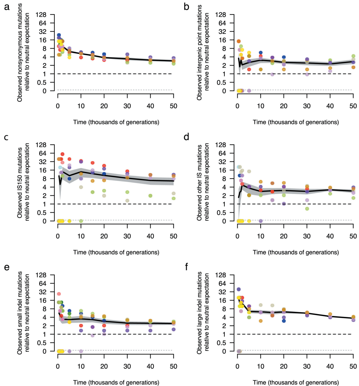
Extended Data Figure 9 | Trajectories for mutations by class in the LTEE in comparison with neutral expectations based on the MAE. a–f , Accumulation of nonsynonymous mutations (a), intergenic point mutations (b), IS150 insertions (c), all other IS-element insertions (d), small indels (e) and large indels (f). Colours are the same as in Fig. 1. All values are expressed relative to the rate at which synonymous mutations accumulated in non-mutator LTEE lineages over 50,000
