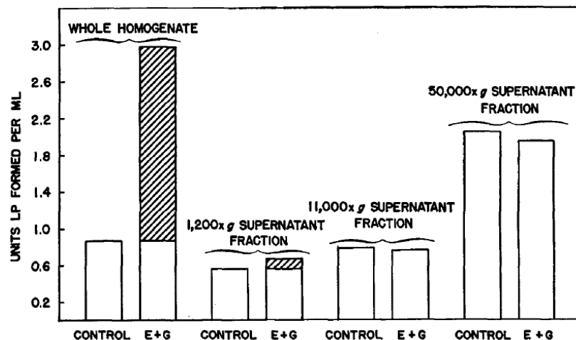
FIG. 3. The effect of epinephrine and glucagon on LP formation in fractions of a cat liver homogenate. 0.14 ml. of homogenate or homogenate fraction was incubated 10 minutes at 30° with 4 \times 10^{-2} M Tris buffer (pH 7.4), 2.5 \times 10^{-3} M MgSO_4 , 1.7 \times 10^{-3} M ATP, and 4.2 units per ml. of dephospho-LP in the presence and absence of 0.4 \gamma of l -epinephrine plus 2.0 \gamma of glucagon. The final volume was 0.20 ml.
