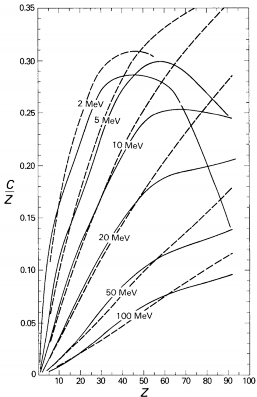
Fig. 3.4. Shell corrections for protons as functions of the atomic number. The solid curves represent the semi-empirical shell corrections of Bichsel, and the dashed curves the theoretical shell corrections of Bonderup (1967). Results are given for various proton energies as indicated.
