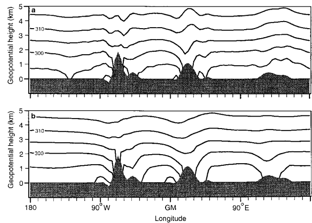
FIG. 13. Longitude–height plots at 24°S showing isentropes in winter (Jun–Aug): (a) from ECMWF analyses for 1983–88 and (b) from day 15 of a model simulation with a Jun–Aug initial state from the same analyses and forced with mountains only. The terrain profile at 24°S is also shown. The contour interval is 5 K.
