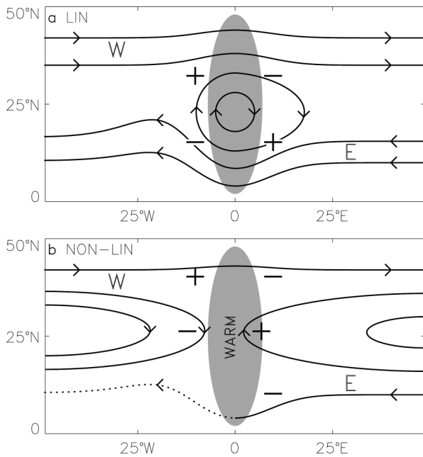
FIG. 12. Schematic diagrams depicting the adiabatic interaction between the zonally averaged flow and an idealized mountain (shaded) based on (a) linear theory in which isentropes do not intersect the mountain in the zonal plane, (b) nonlinear theory in which isentropes can intersect the mountain in the zonal plane. Contours depict low-level streamfunction. Here “+” indicates ascent and “-” indicates descent.
