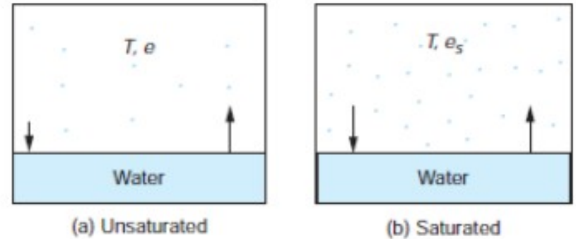
Fig. 3.8 A box (a) unsaturated and (b) saturated with respect to a plane surface of pure water at temperature T . Dots represent water molecules. Lengths of the arrows represent the relative rates of evaporation and condensation. The saturated (i.e., equilibrium) vapor pressure over a plane surface of pure water at temperature T is e_s , as indicated in (b).
