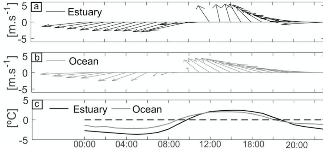
Figure 4: Daily cycle of winds [ \text{m}\cdot\text{s}^{-1} ] during summer in: a) Estuary and b) Ocean. c) Difference between air and water temperature [ \Delta T , ^{\circ}\text{C} ] in the estuary and oceanic region during summer, respectively. Wind data and air temperature from all estuarine and oceanic stations were used to compute each panel respectively. For the SST, representative time series for each region was taken (see methods).
