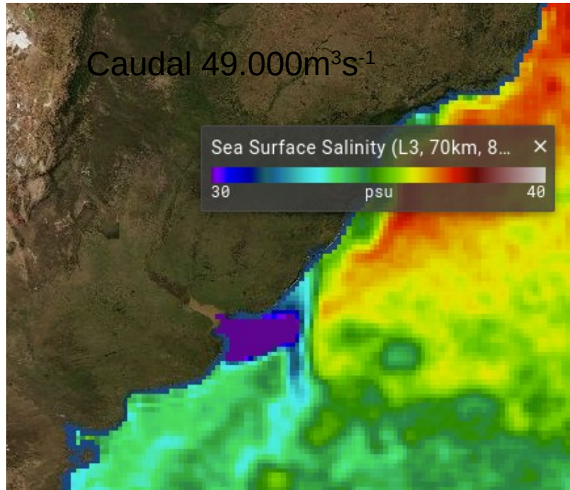
SMAP/REMSS 17/02/2016
