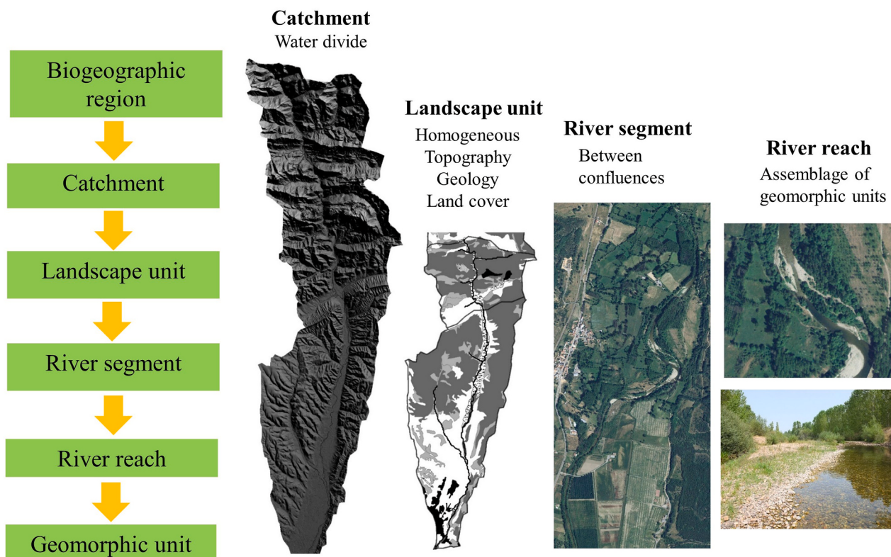
Fig. 2. Multi-scale hierarchical approach for hydromorphological studies, developed within the REFORM Project (Gurnell et al., 2016a) and proposed to characterize and assess riparian vegetation at multiple spatial scales.
