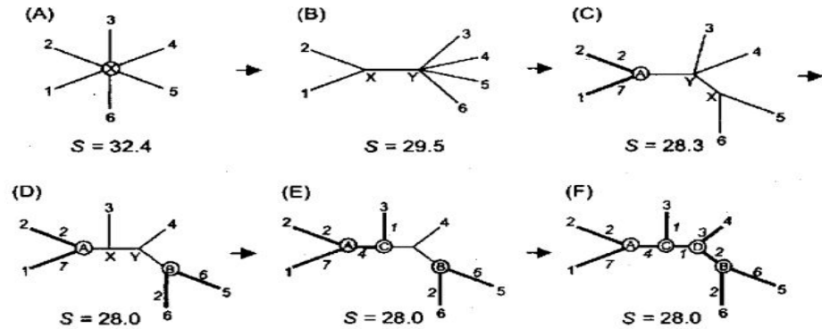
FIGURE 6.7. Illustration of the computational process in the neighbor-joining method.
