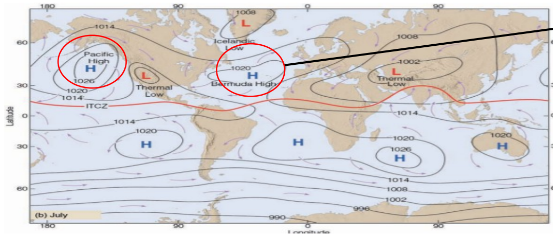
Sea level pressure distribution and Surface wind flow patterns
