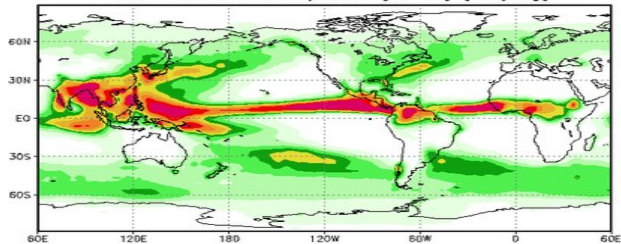
Mean JJA GPCP Precipitation (79-03) (mm/day)
