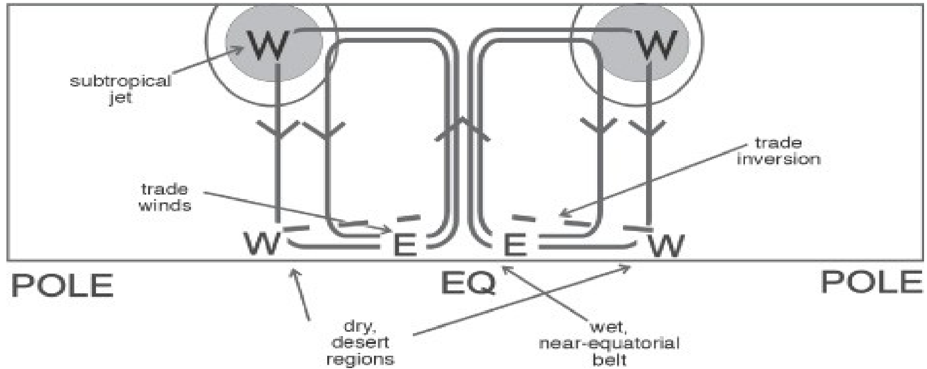
Figure 8.5: A schematic diagram of the Hadley circulation and its associated zonal flows and surface circulation.
