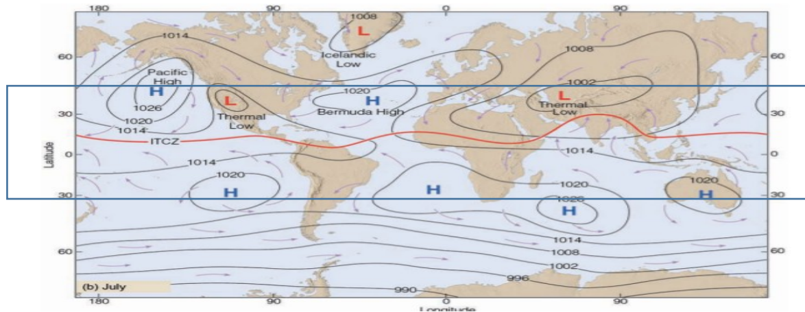
Sea level pressure distribution and Surface wind flow patterns
