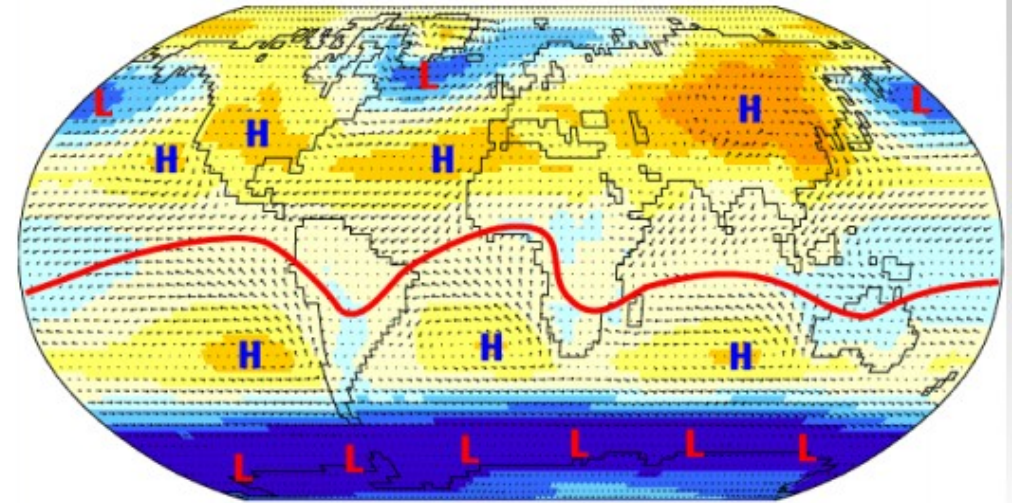
995 1000 1005 1010 1015 1020 1025 mb Sea-Level Pressure and Surface Winds
