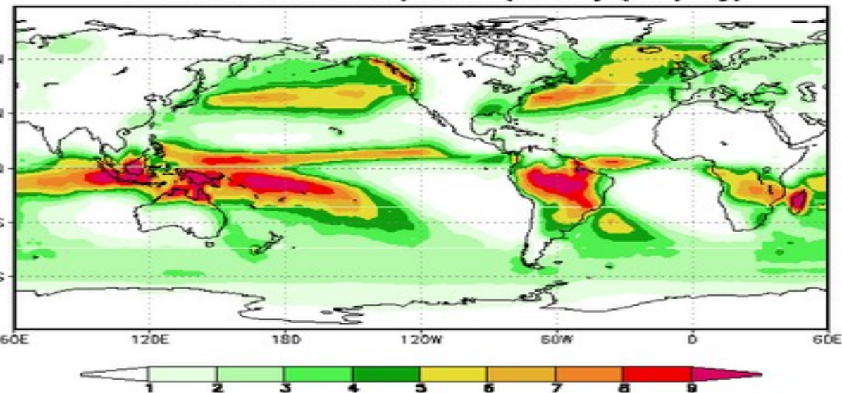
Mean DJF GPCP Precipitation (79-03) (mm/day)
