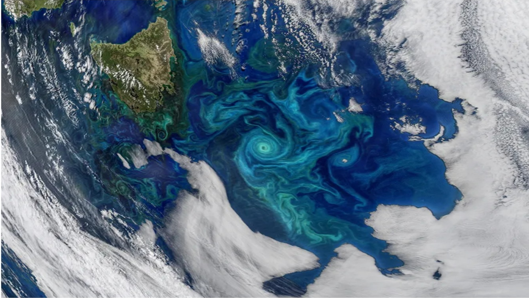
Phytoplankton bloom in the Tasman Sea captured by the NASA Moderate Resolution Imaging Spectroradiometer (MODIS) instrument on the Aqua satellite on 21 November 2017. White patches are clouds. Advances in remote and in situ sensing, as well as methods for modeling and simulation, are driving an era of progress in ocean biogeochemistry research. Credit: NASA/Ocean Biology Processing Group, Goddard Space Flight Center
