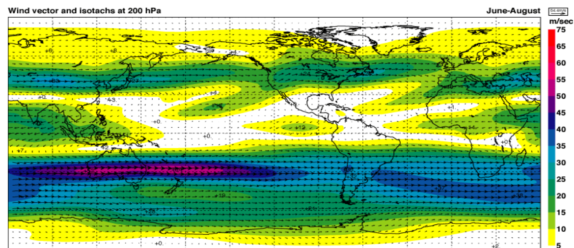
Wind vector and isotachs at 200 hPa
