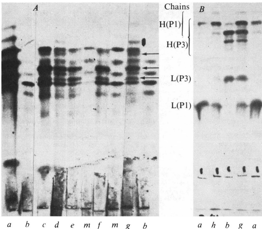
Fig. 1 Autoradiograph of labelled components secreted by the parental and hybrid cell lines analysed by IEF before (A) and after reduction (B). Cells were incubated in the presence of 14 C-lysine 14 and the supernatant applied on polyacrylamide slabs. A, pH range 6.0 (bottom) to 8.0 (top) in 4 M urea. B, pH range 5.0 (bottom) to 9.0 (top) in 6 M urea; the supernatant was incubated for 20 min at 37 °C in the presence of 8 M urea, 1.5 M mercaptoethanol and 0.1 M potassium phosphate pH 8.0 before being applied to the right slab. Supernatants from parental cell lines in: a, P1Bu1; b, P3-X67Ag8; and m, mixture of equal number of P1Bu1 and P3-X67Ag8 cells. Supernatants from two independently derived hybrid lines are shown: c-f, four subclones from Hy-3; g and h, two subclones from Hy-B. Fusion was carried out 14,9 using 10 6 cells of each parental line and 4,000 haemagglutination units inactivated Sendai virus (Searle). Cells were divided into ten equal samples and grown separately in selective medium (HAT medium, ref. 6). Medium was changed every 3 d. Successful hybrid lines were obtained in four of the cultures, and all gave similar IEF patterns. Hy-B and Hy-3 were further cloned in soft agar 14 . L, Light; H, heavy.
