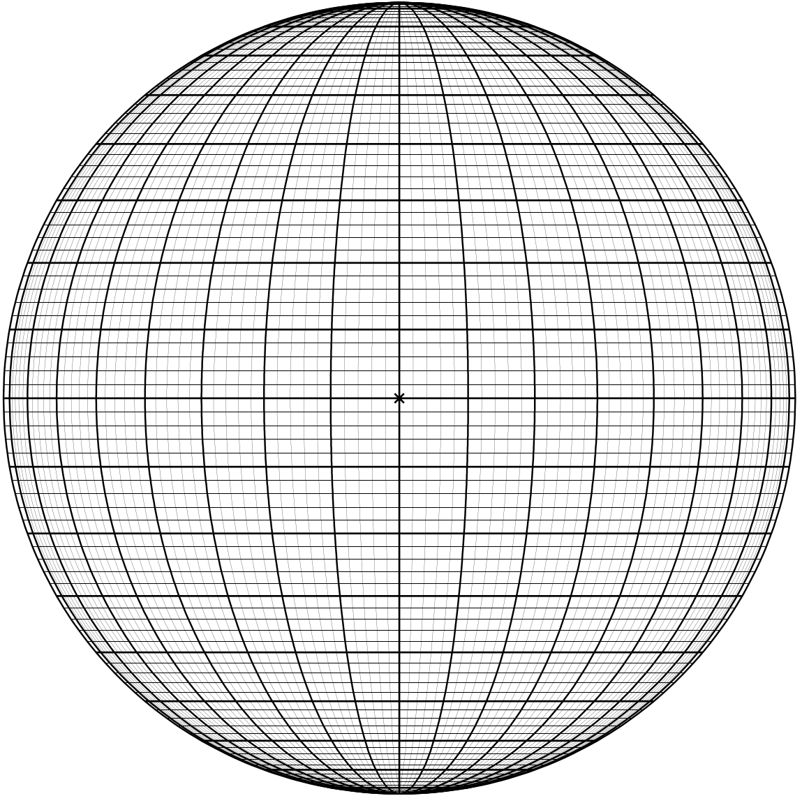
Orthographic net
