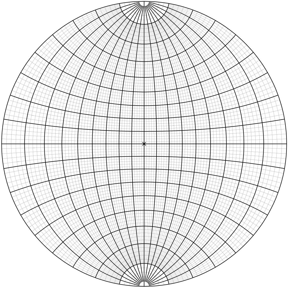
Stereonet
