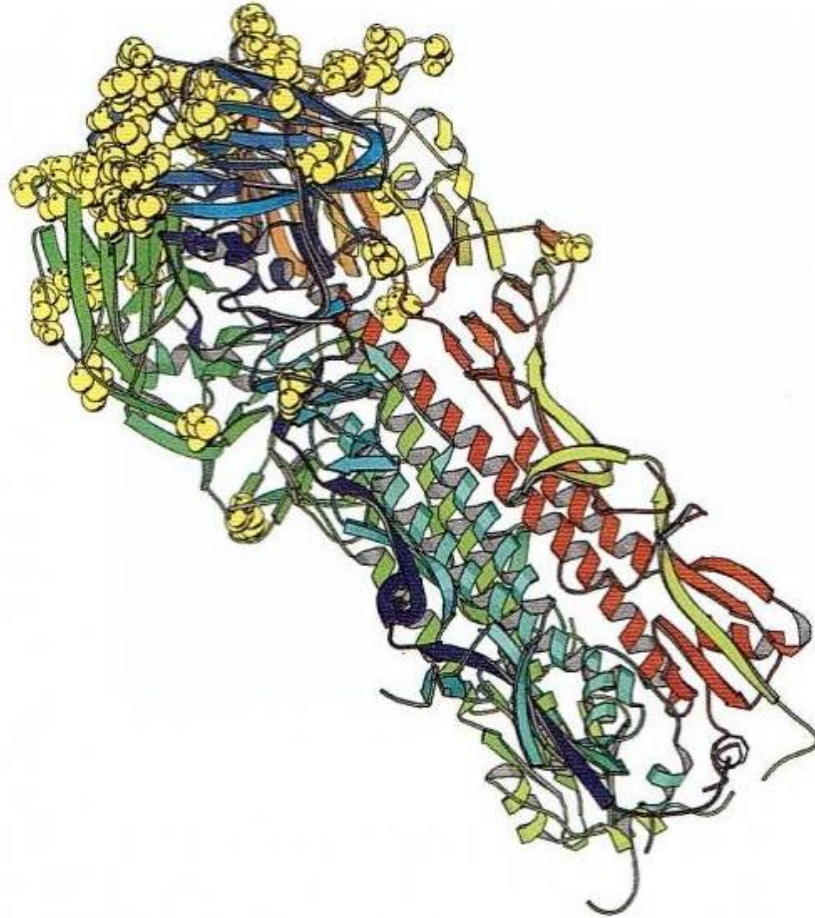
FIGURE 16.10 Model of the Hemagglutinin Protein, Showing Amino Acid Sites that Are Under Positive Selection for Change (Yellow Spheres) From Hillis 1999a.
