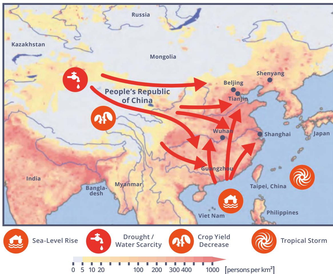
Figure 20. Climate impacts and possible migration routes in China 2100 (Image: ADB 28 ).
