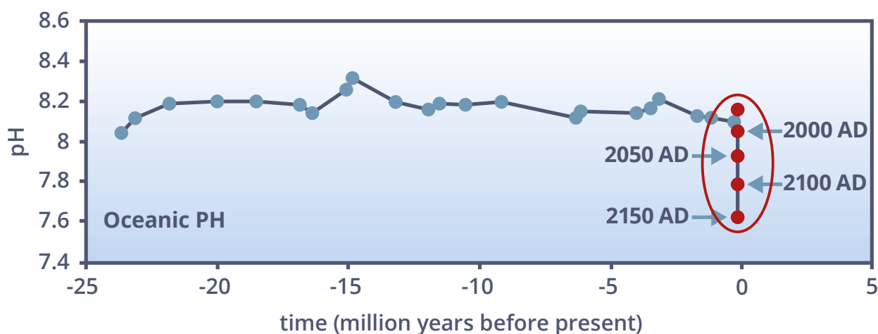
Figure 9. The changes in ocean pH over the last 25 million years. Significant changes are now occurring at a rate and to a level not experienced by marine organisms for around 60 million years (Source: Carol Turley)
